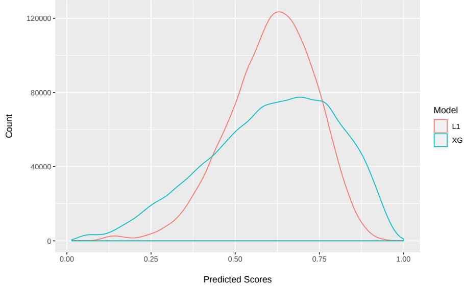
Figure 1: Score Densities . The figure compares the distributions of the scores predicted by two scoring models: L1-regularized logistic regression (red) and extreme gradient boosting (blue). Both models use the same data.
