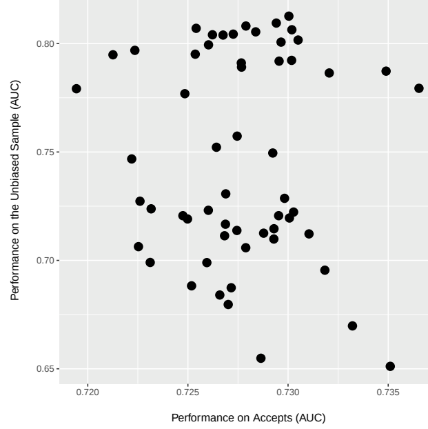
Figure 2: Comparing AUC on the accepted cases (4-fold cross-validation) and the unbiased sample. The dots indicate scoring models with different meta-parameters.
