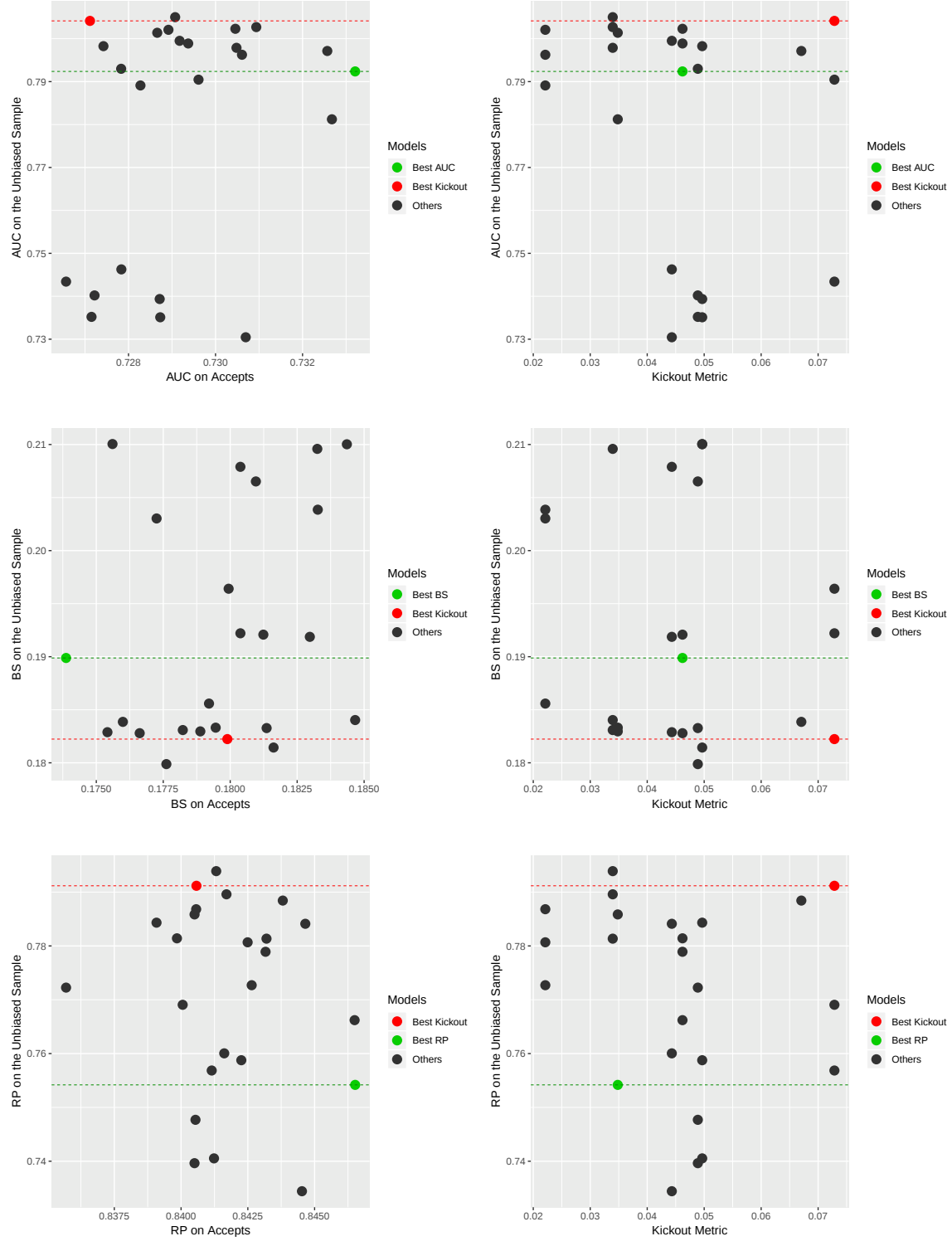
Figure 3: Model Selection Results. Two upper diagrams compare model selection results based on AUC on the accepted cases (green) and on the kickout metric (red). Two diagrams in the center compare results based on Brier Score on the accepts (green) and the kickout metric (red), whereas two lower diagrams refer to R-Precision on the accepts (green) and kickout (red).
